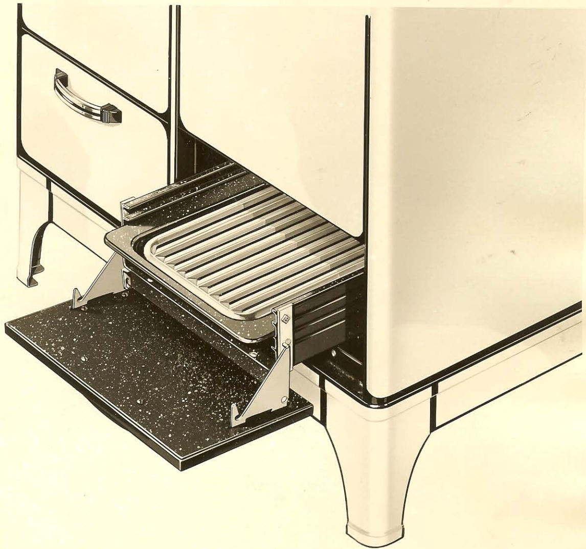
PARAMOUNT MODEL 6E6 EQUIPPED WITH "HI-EFFICIENCY" BROILER AND DROP FRONT BROILER DOOR
